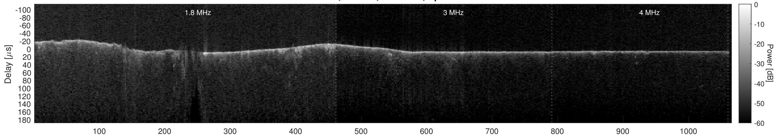
Orbit 5987, Cluttergram
