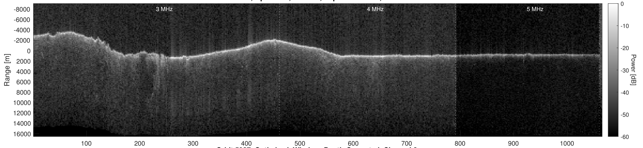
Orbit 5987, Optimized, Window, Depth-Corrected, Channel 2
