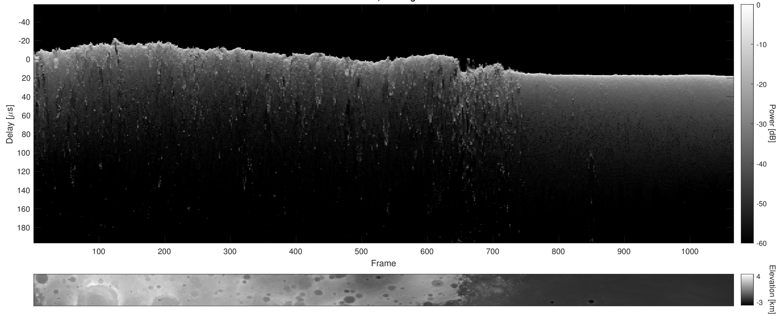
Orbit 5988, Cluttergram
