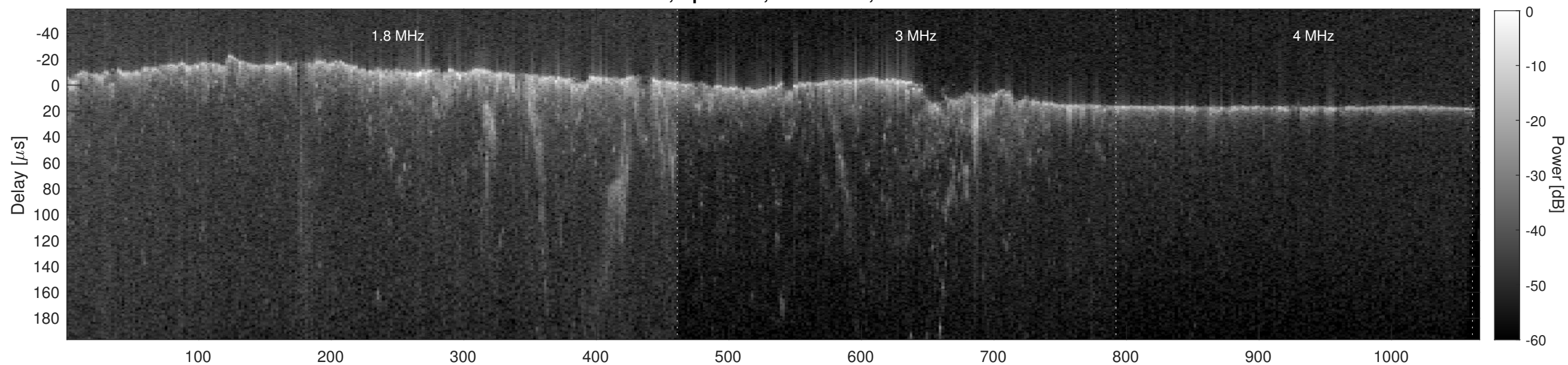
Orbit 5988, Cluttergram
