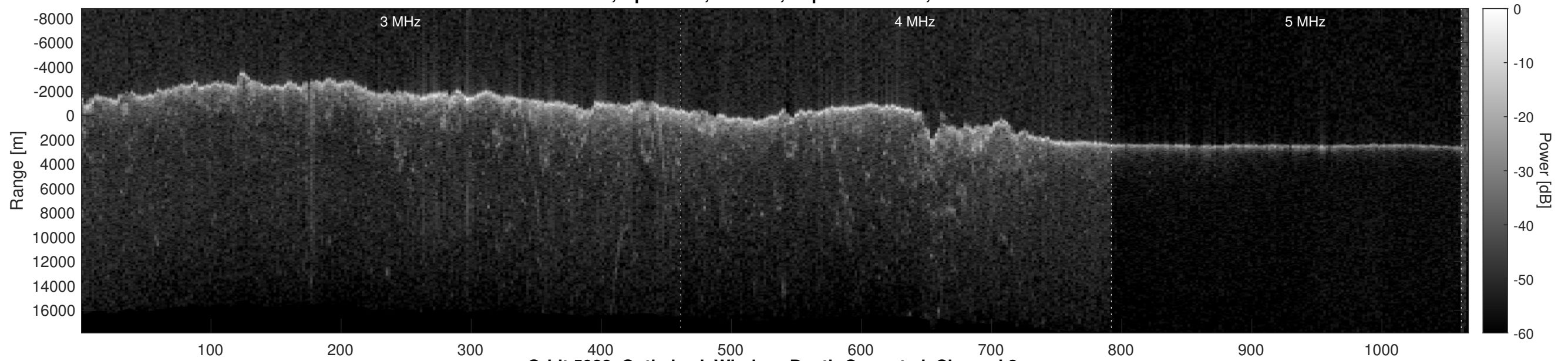
Orbit 5988, Optimized, Window, Depth-Corrected, Channel 2
