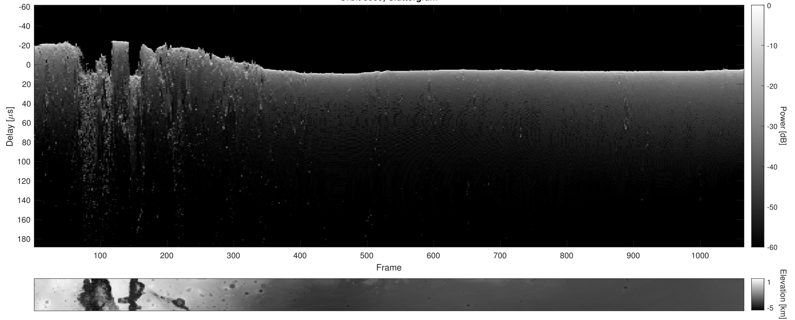
Orbit 5989, Cluttergram
