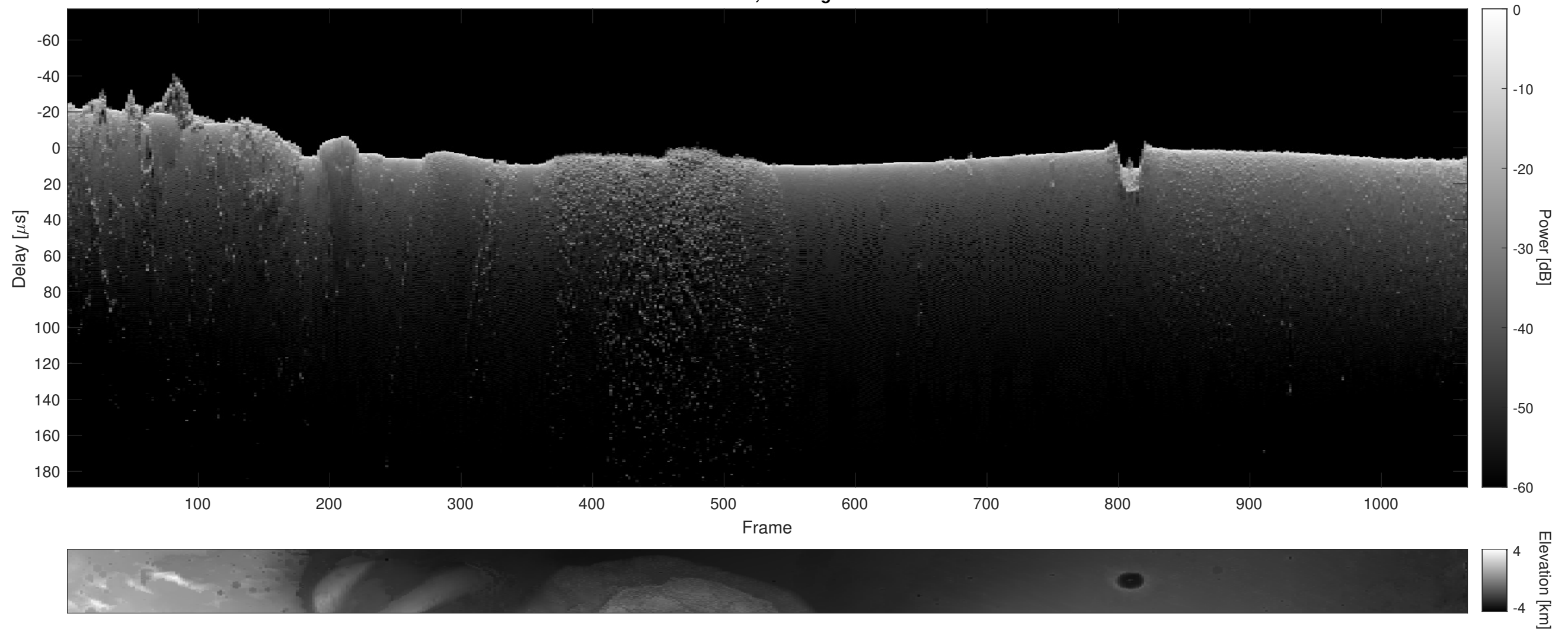
Orbit 5990, Cluttergram
