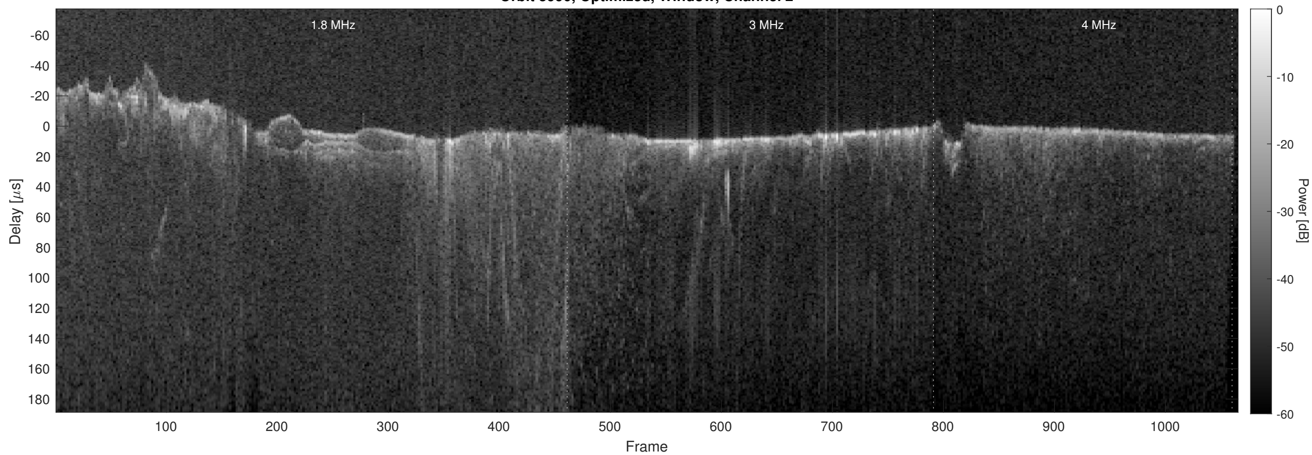
Orbit 5990, Optimized, Window, Channel 2
