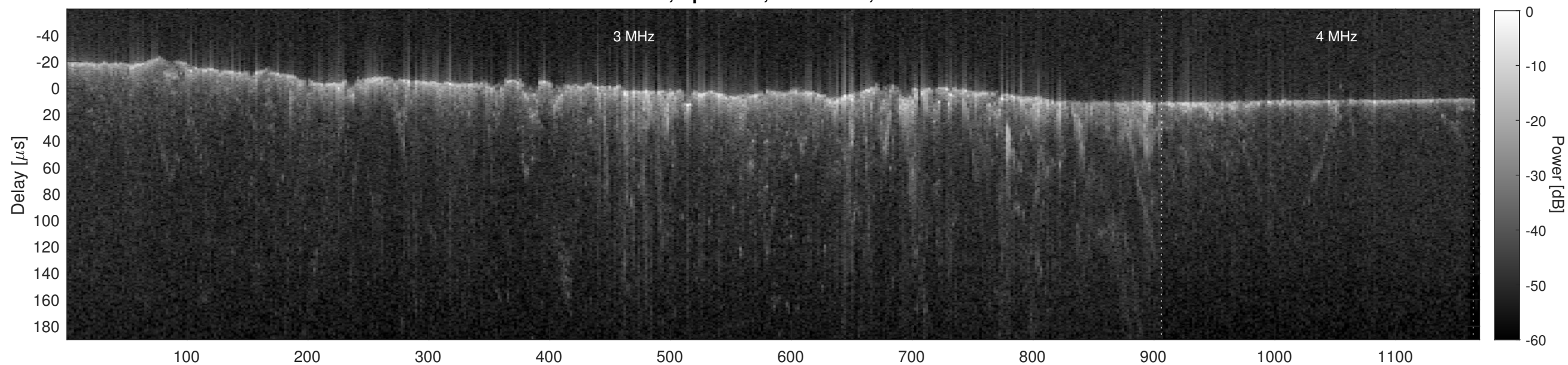
Orbit 5992, Cluttergram
