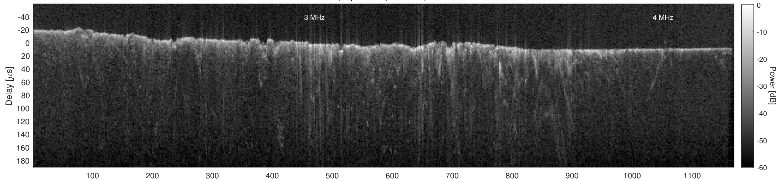
Orbit 5992, Cluttergram
