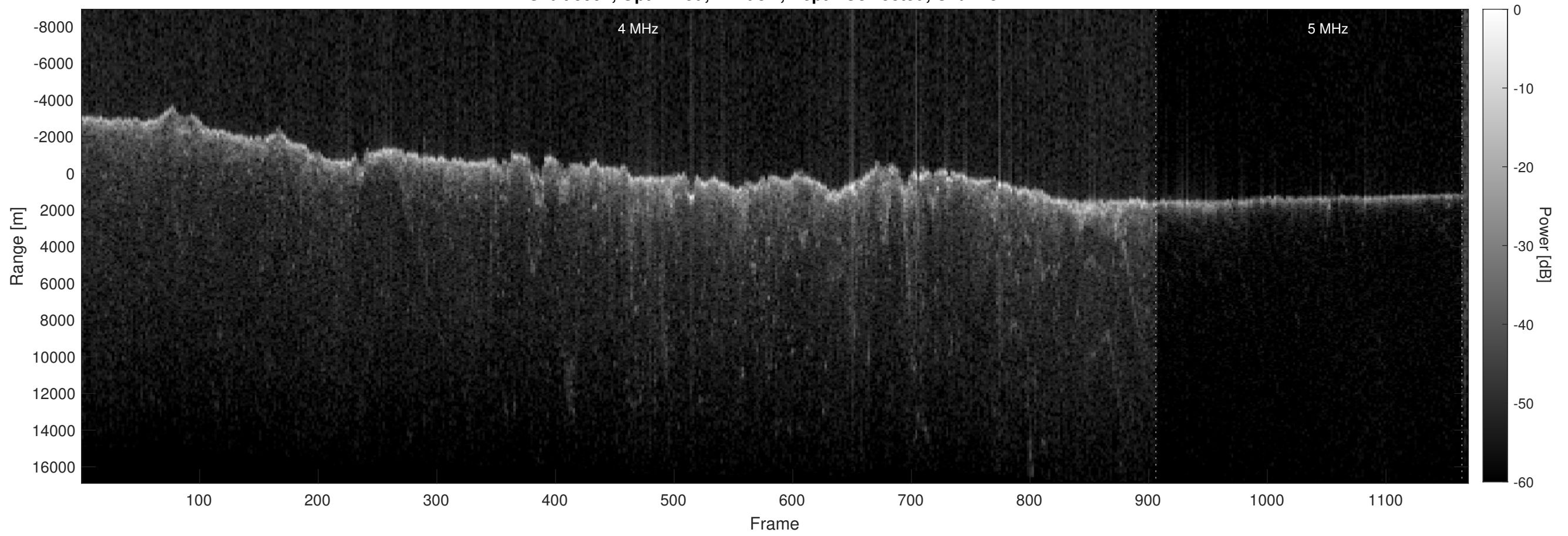
Orbit 5992, Optimized, Window, Depth-Corrected, Channel 2
