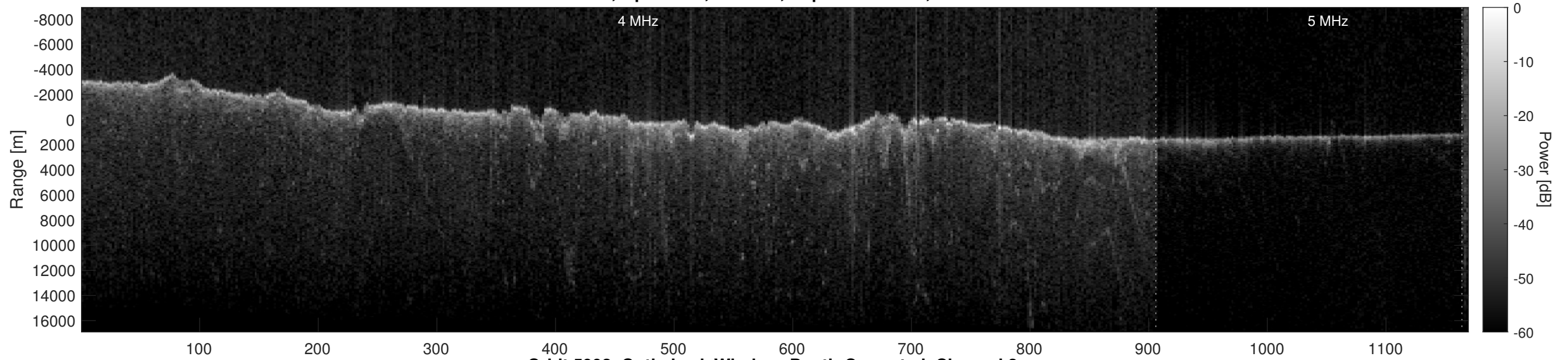
Orbit 5992, Optimized, Window, Depth-Corrected, Channel 2
