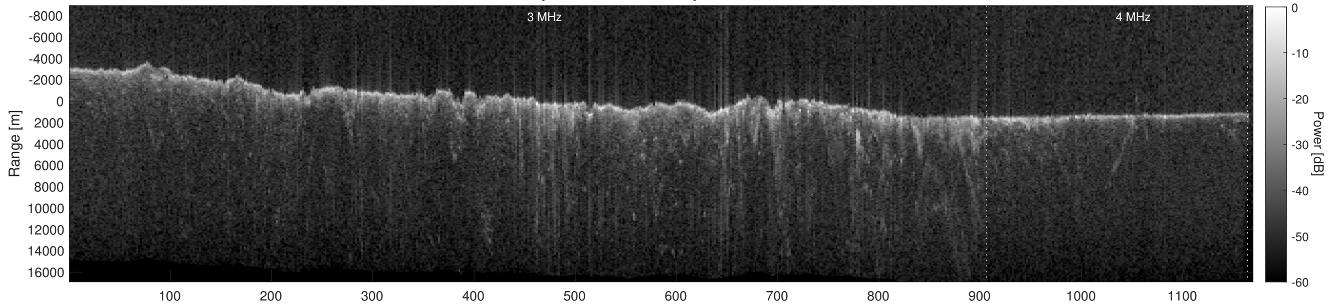
Orbit 5992, Depth-Corrected Cluttergram
