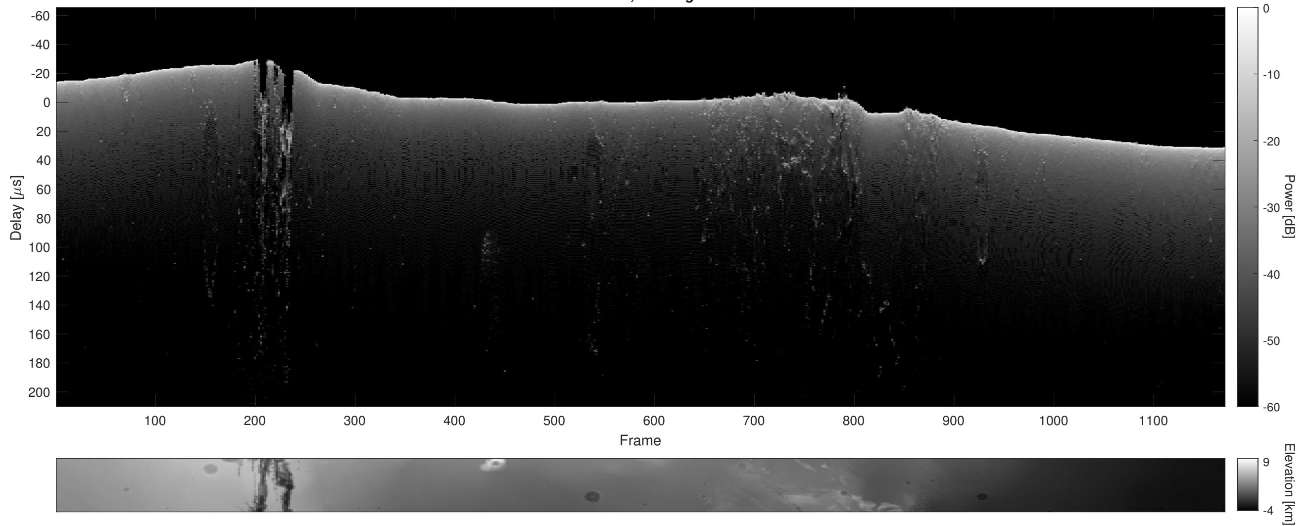
Orbit 5993, Cluttergram
