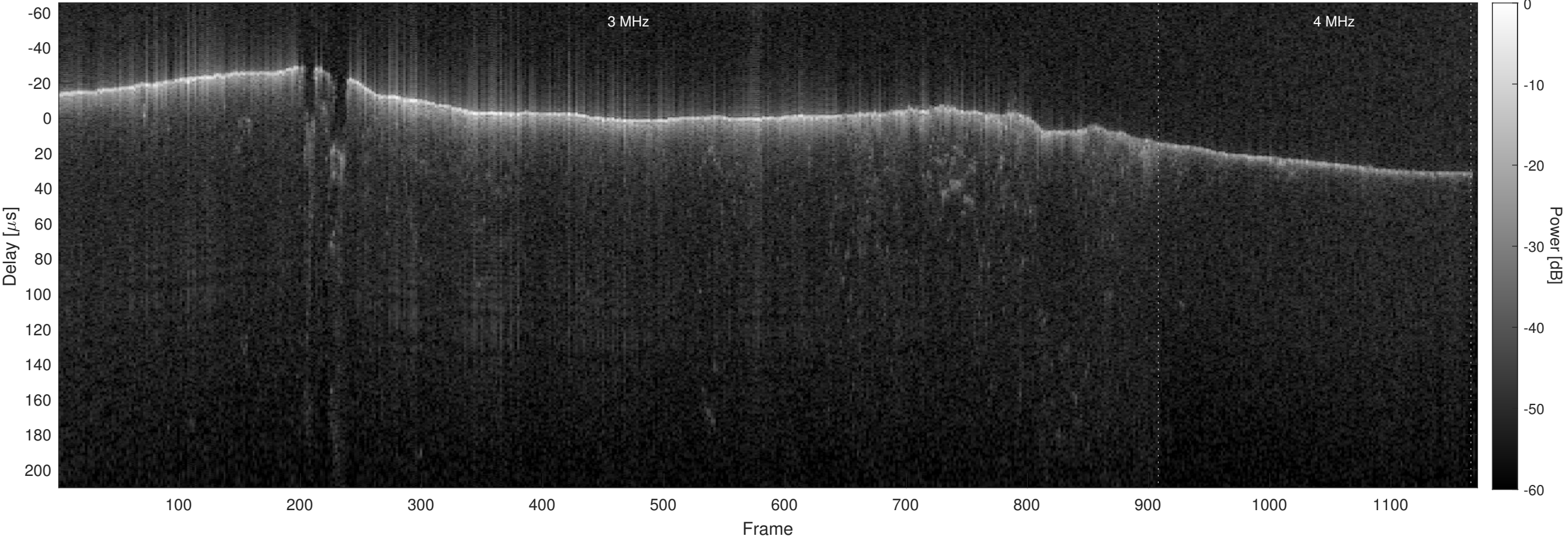
Orbit 5993, Optimized, No Window, Channel 2
