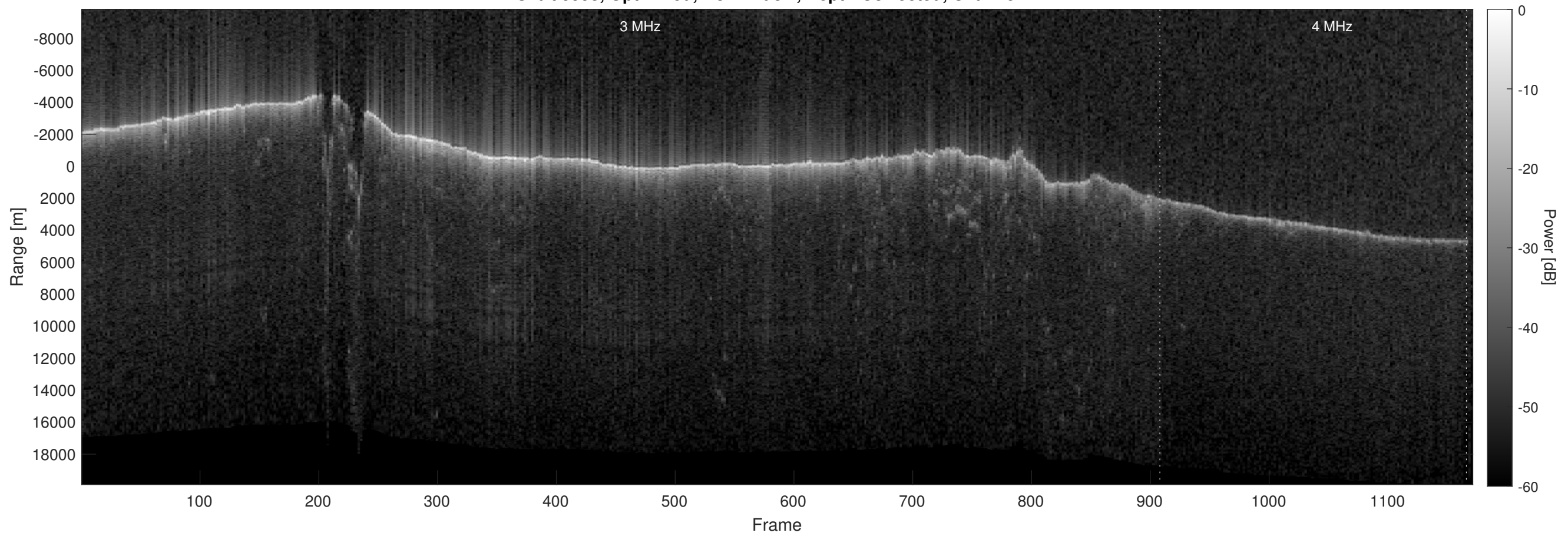
Orbit 5993, Optimized, No Window, Depth-Corrected, Channel 2
