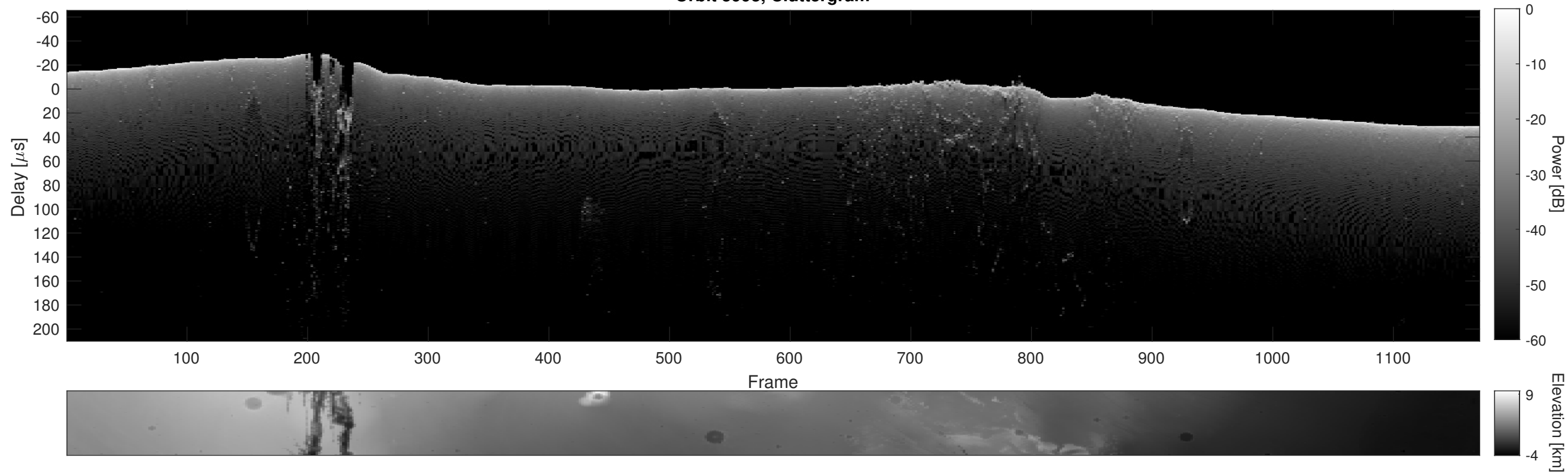
Orbit 5993, Cluttergram
