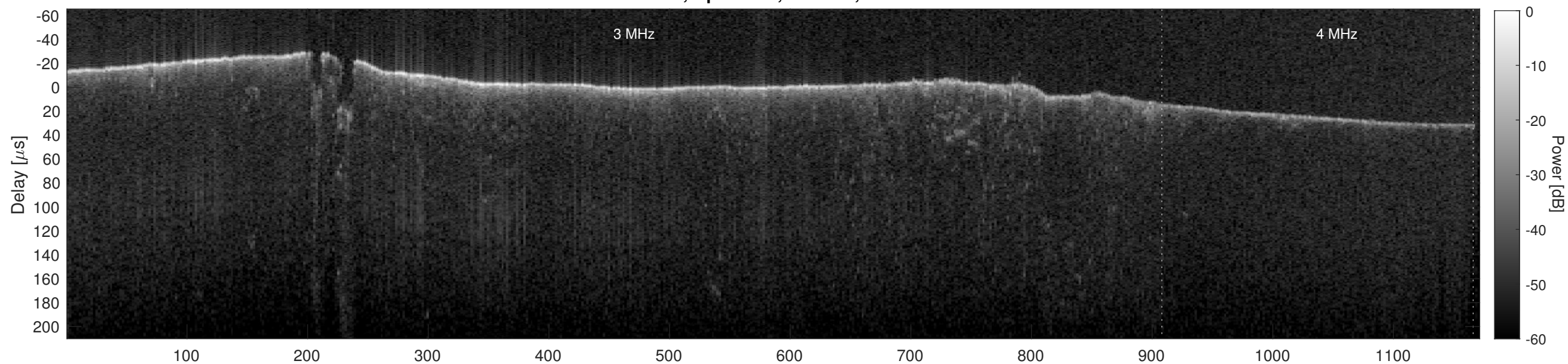
Orbit 5993, Cluttergram
