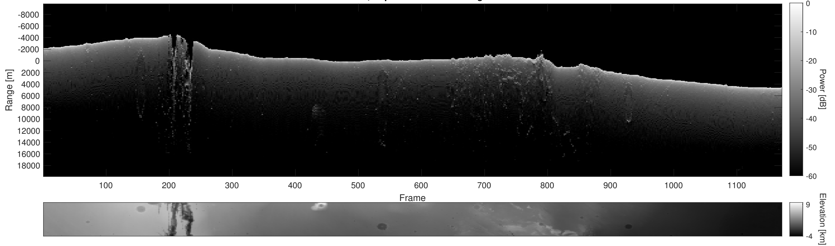
Orbit 5993, Depth-Corrected Cluttergram
