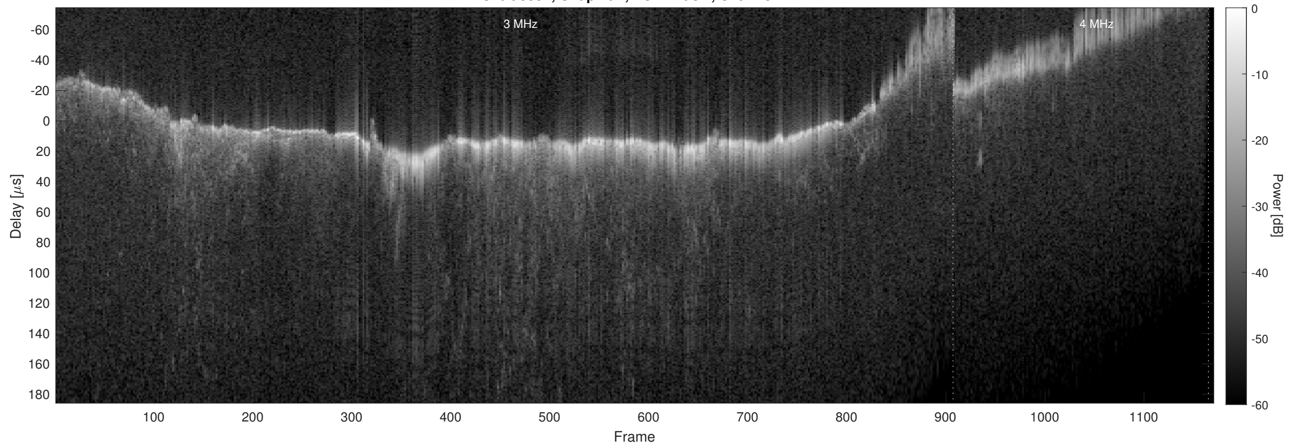
Orbit 5994, Chapman, No Window, Channel 2
