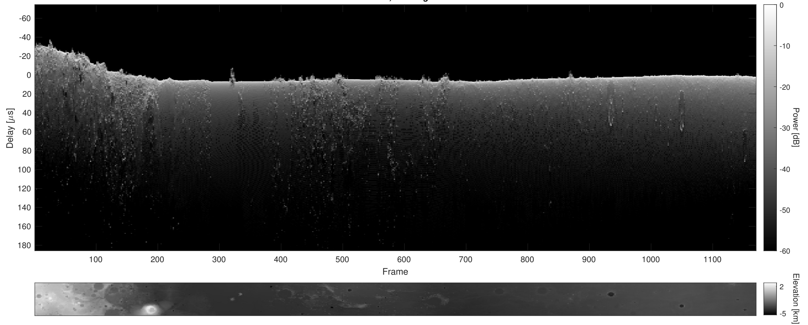
Orbit 5994, Cluttergram
