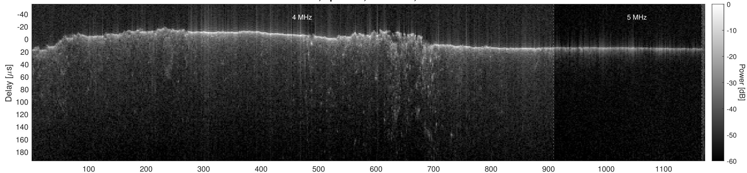
Orbit 5995, Optimized, No Window, Channel 2
