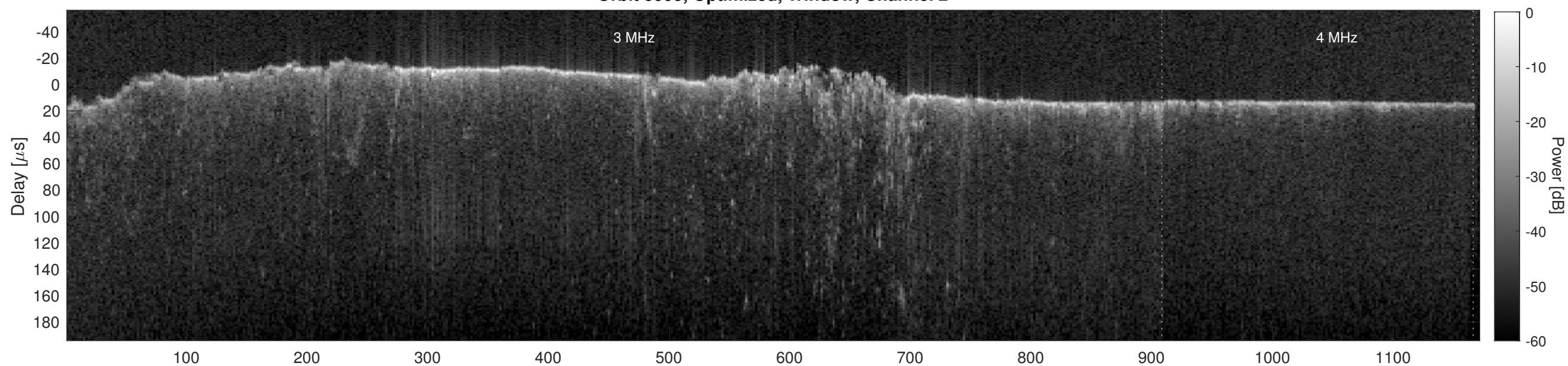
Orbit 5995, Cluttergram
