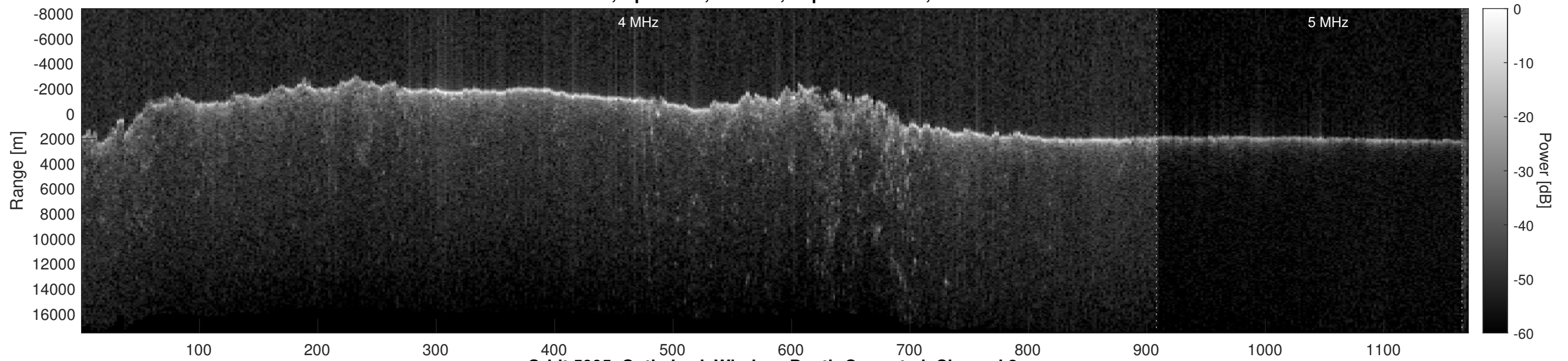
Orbit 5995, Optimized, Window, Depth-Corrected, Channel 2
