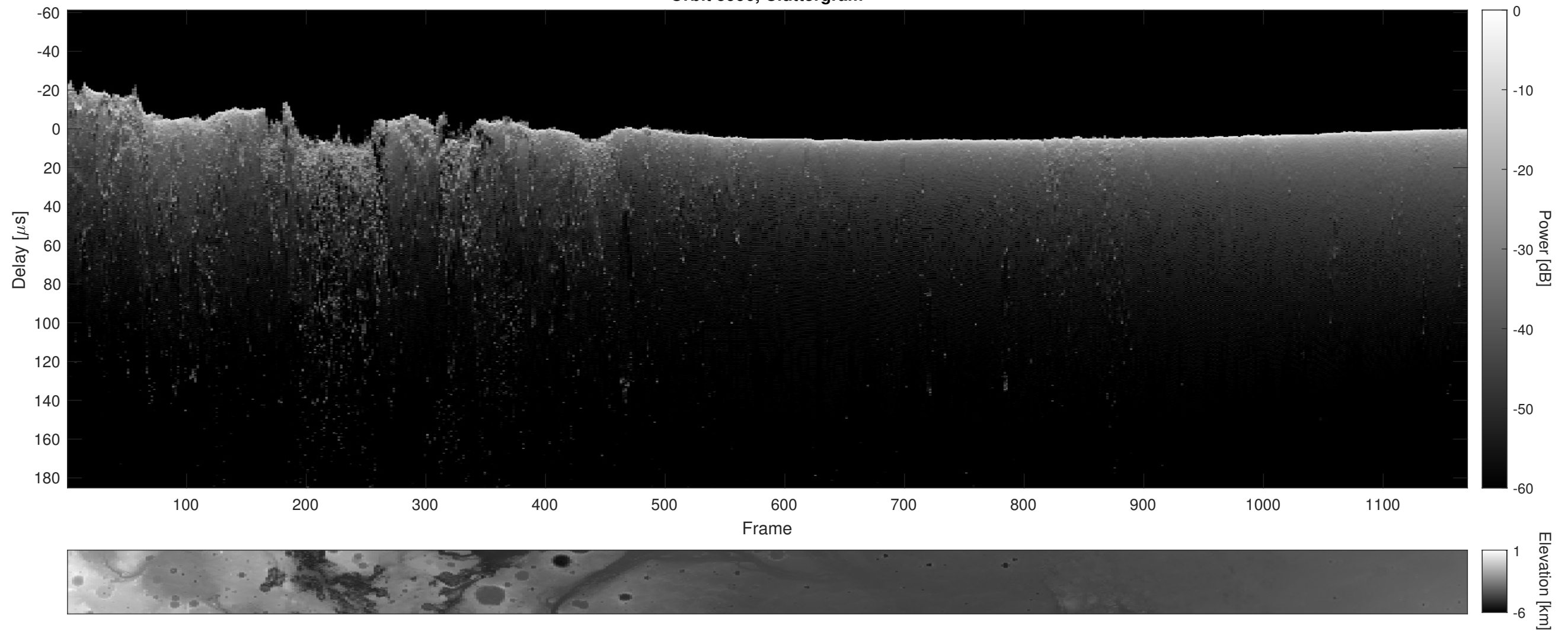
Orbit 5996, Cluttergram
