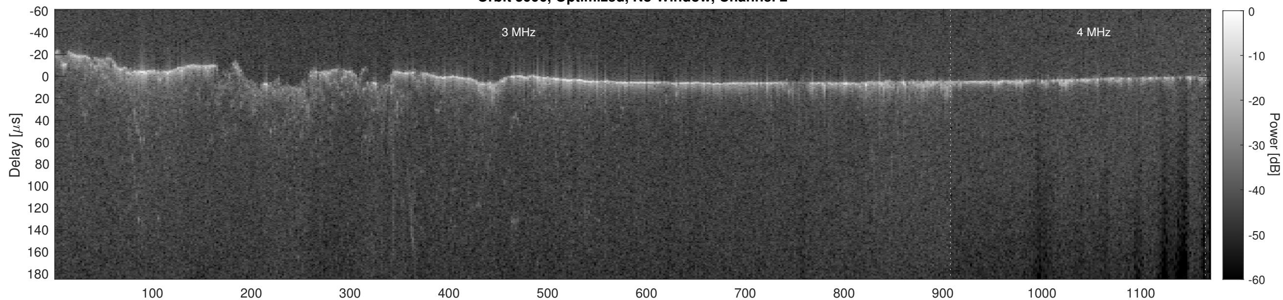
Orbit 5996, Cluttergram
