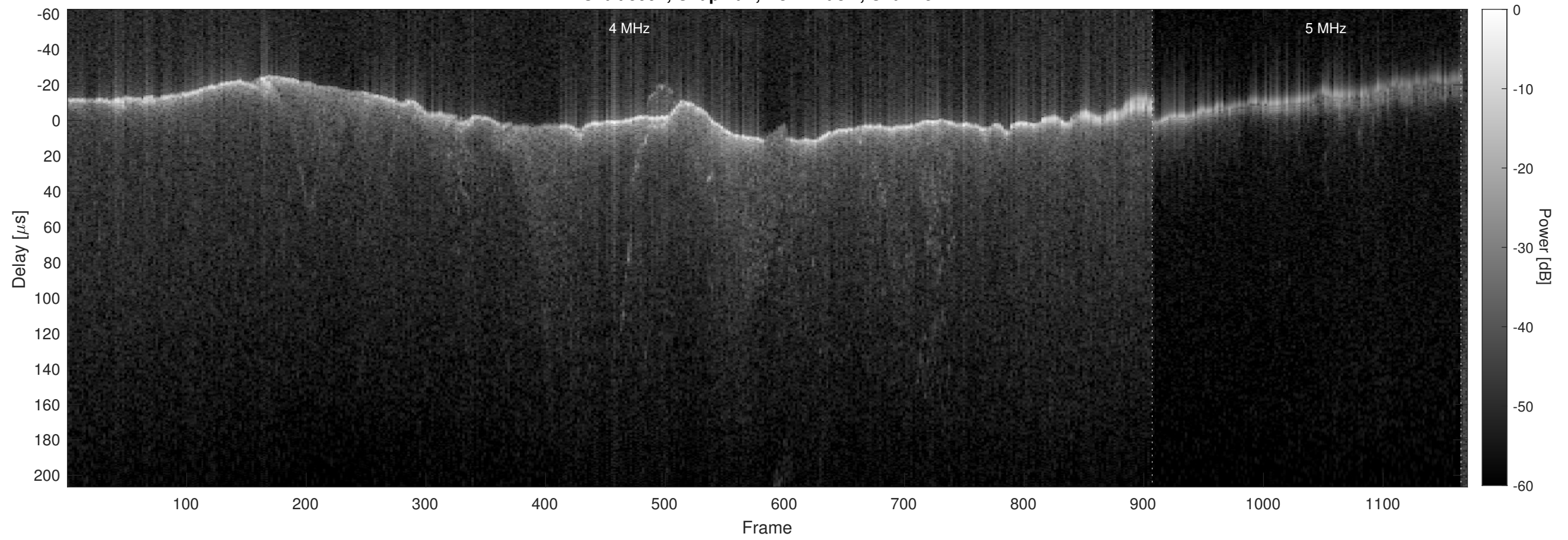
Orbit 5997, Chapman, No Window, Channel 2
