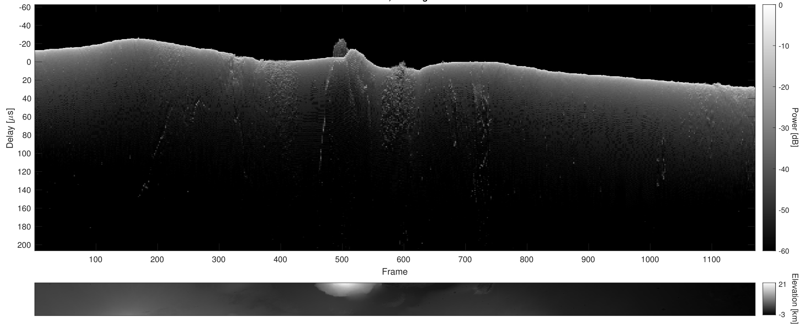
Orbit 5997, Cluttergram
