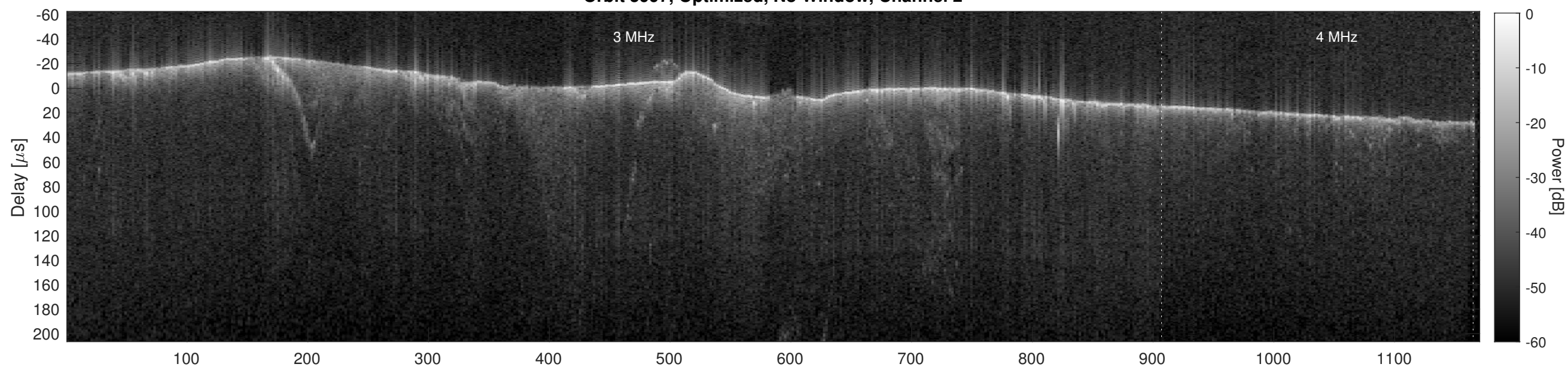
Orbit 5997, Cluttergram
