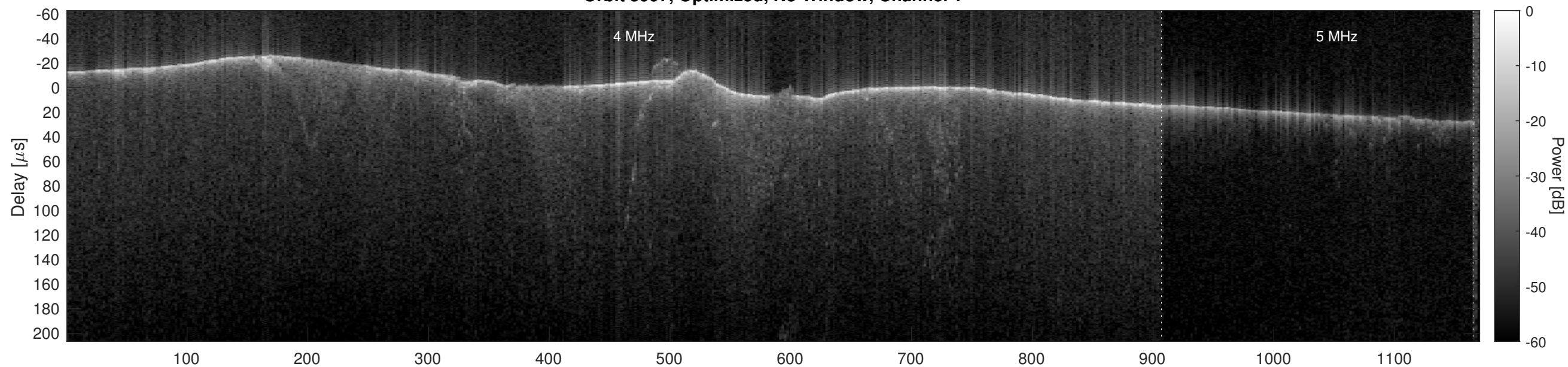
Orbit 5997, Optimized, No Window, Channel 2
