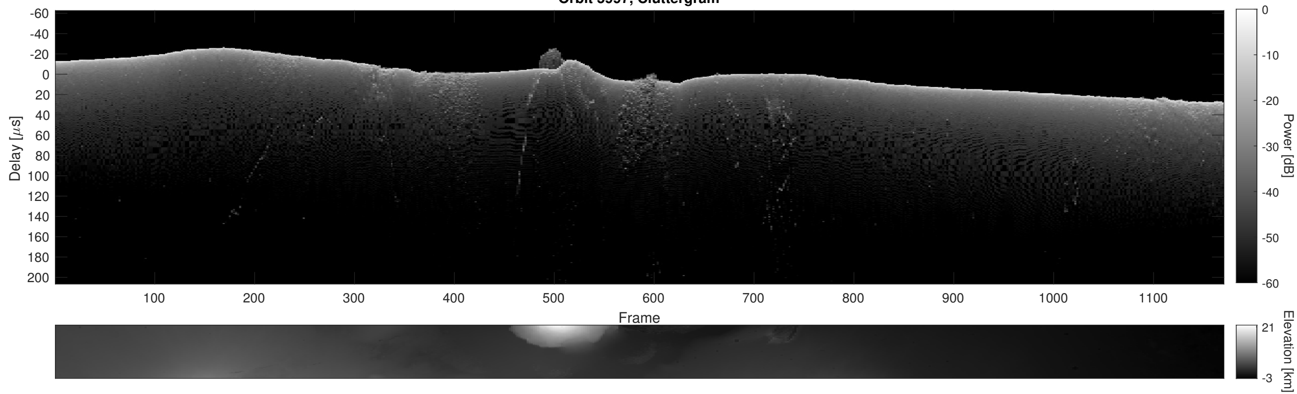
Orbit 5997, Cluttergram
