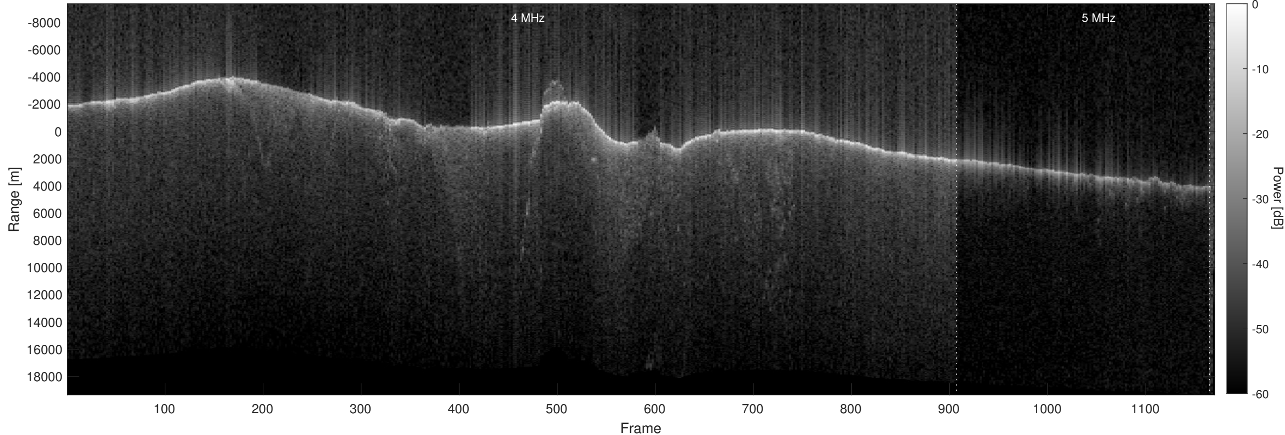
Orbit 5997, Optimized, No Window, Depth-Corrected, Channel 2
