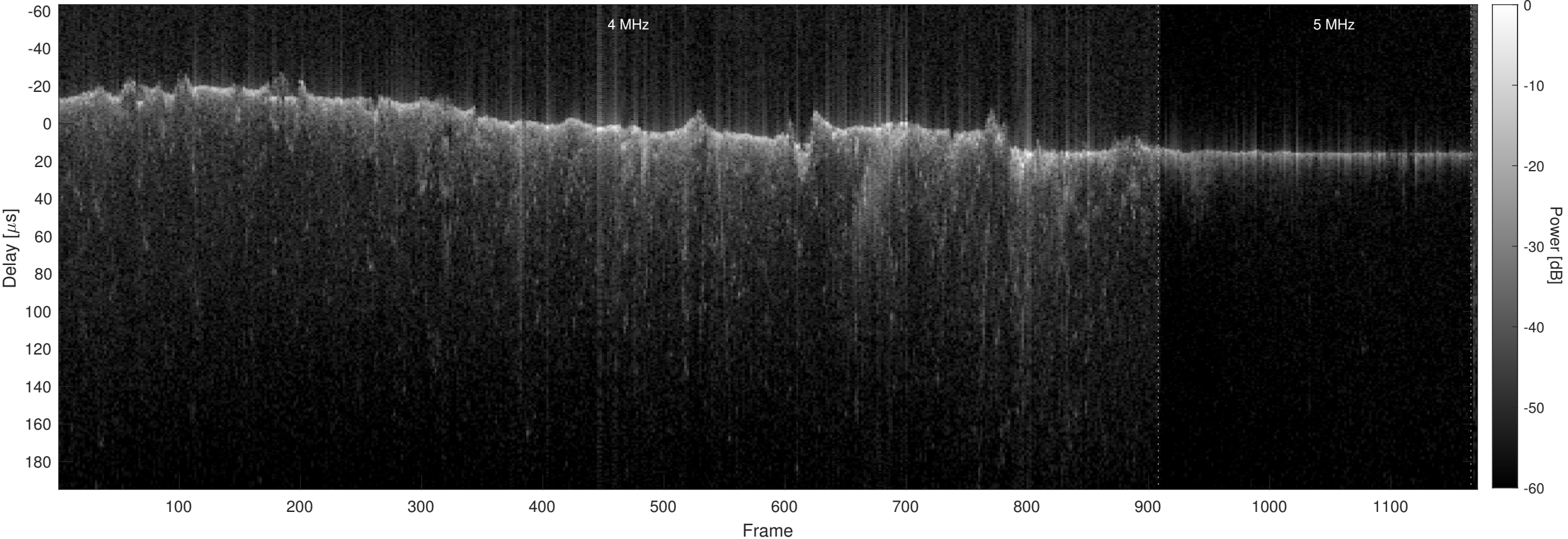
Orbit 5999, Optimized, No Window, Channel 2
