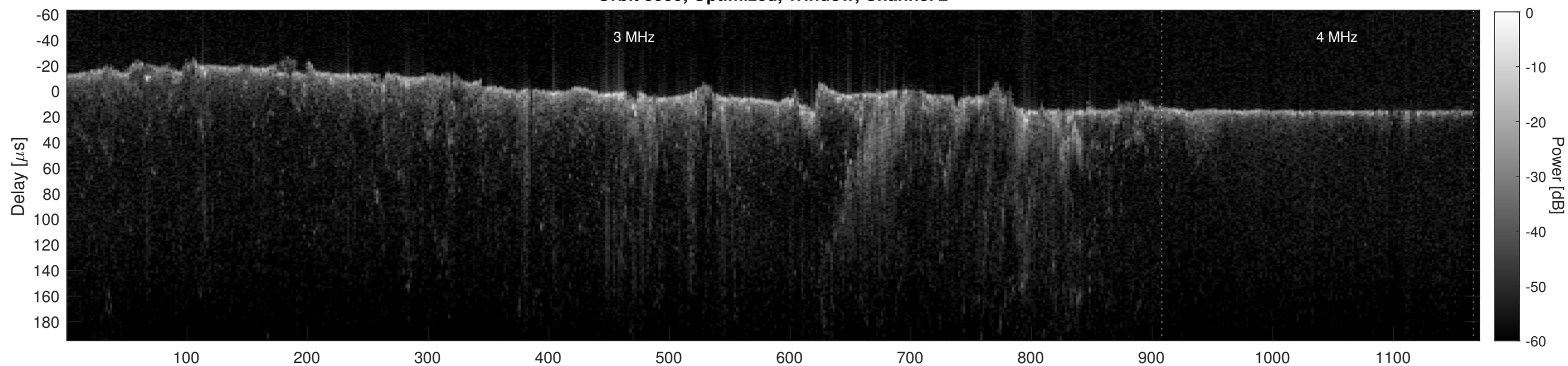
Orbit 5999, Cluttergram
