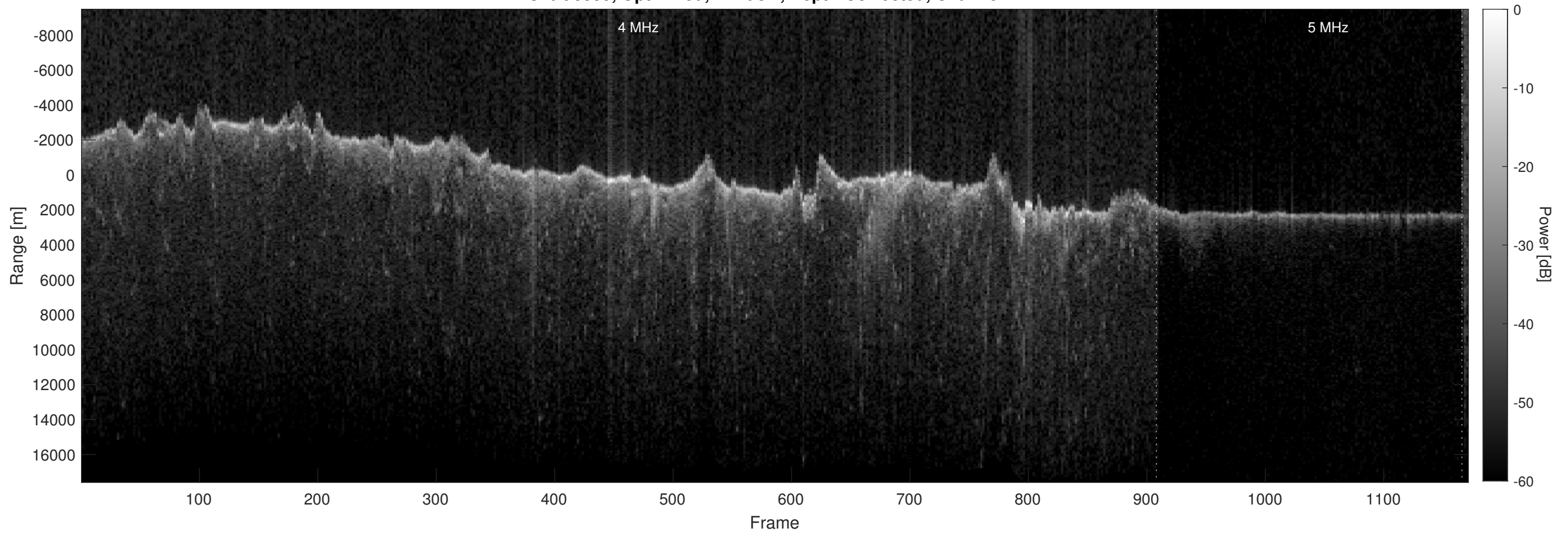
Orbit 5999, Optimized, Window, Depth-Corrected, Channel 2
