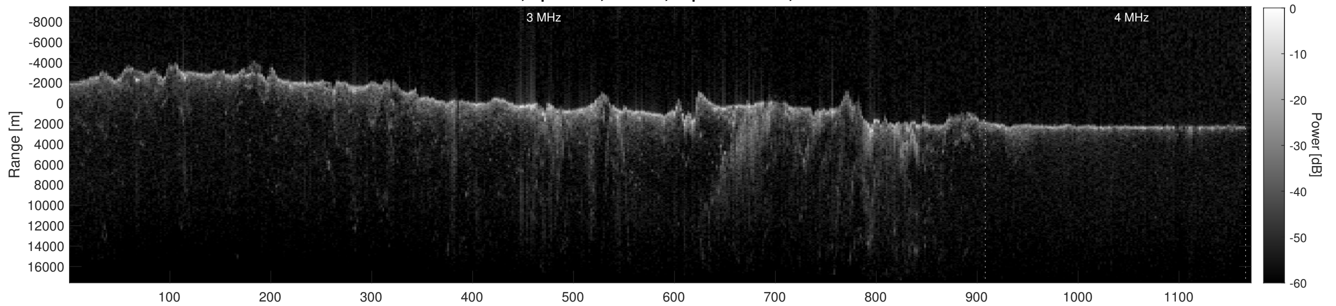
Orbit 5999, Depth-Corrected Cluttergram
