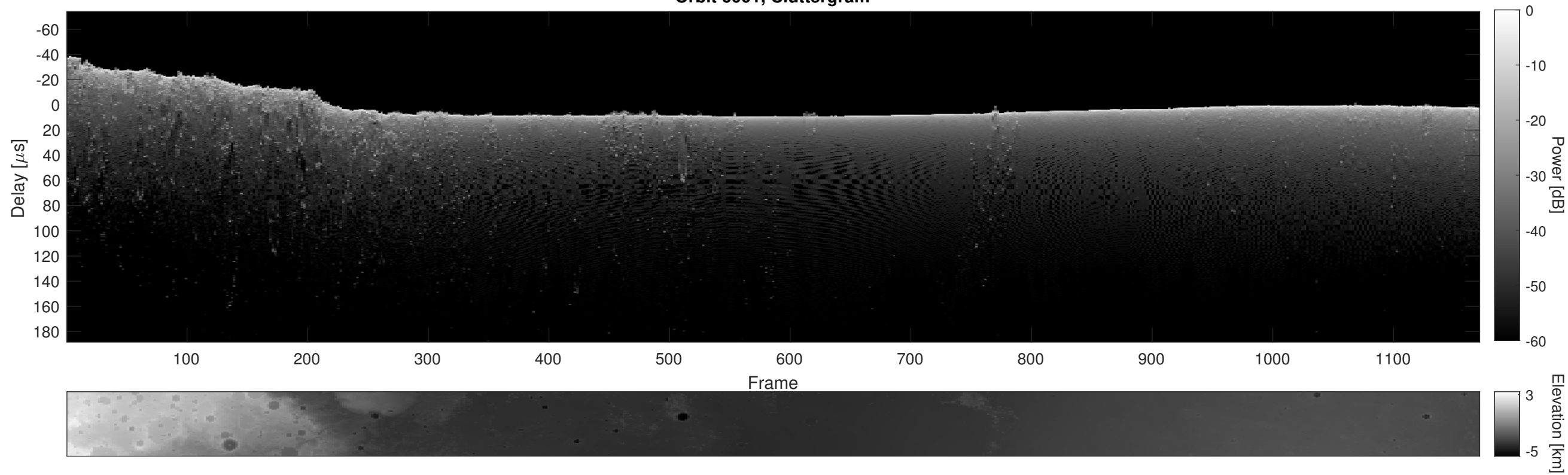
Orbit 6001, Cluttergram
