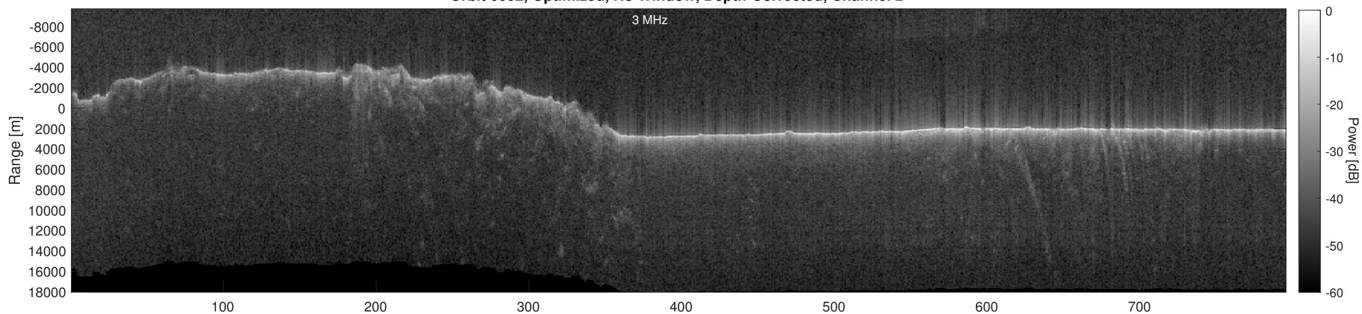
Orbit 6002, Depth-Corrected Cluttergram
