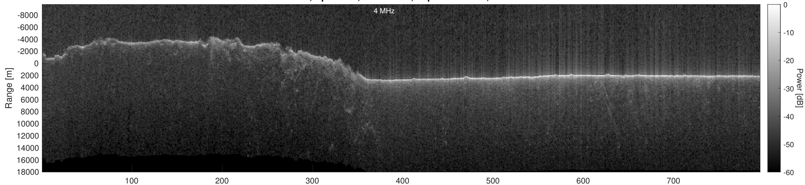
Orbit 6002, Optimized, No Window, Depth-Corrected, Channel 2
