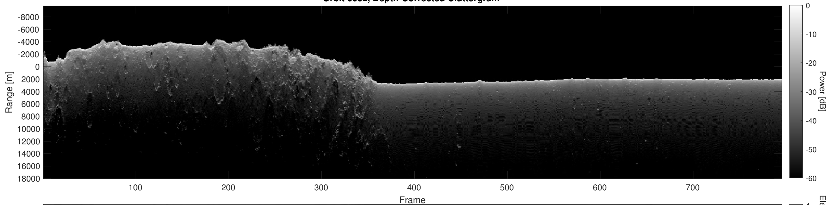
Orbit 6002, Depth-Corrected Cluttergram
