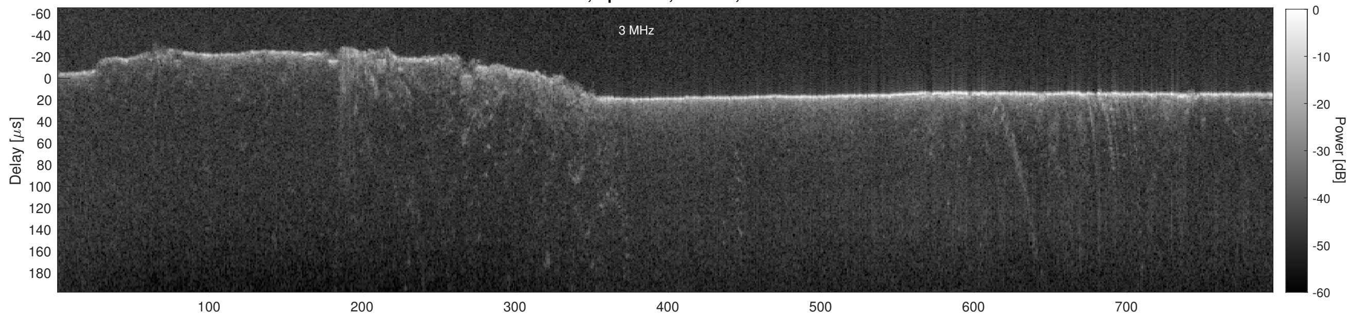
Orbit 6002, Cluttergram
