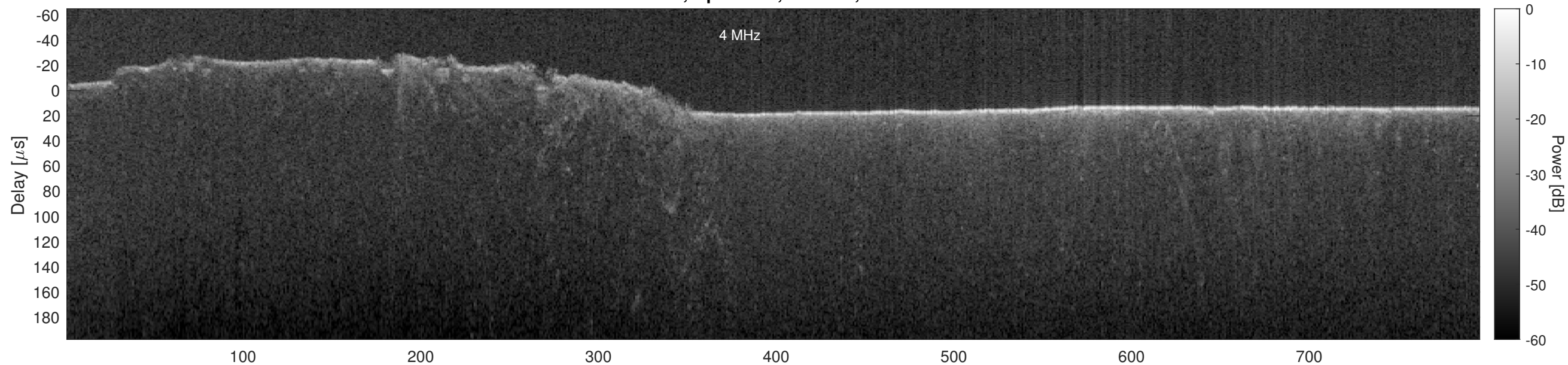
Orbit 6002, Optimized, Window, Channel 2
