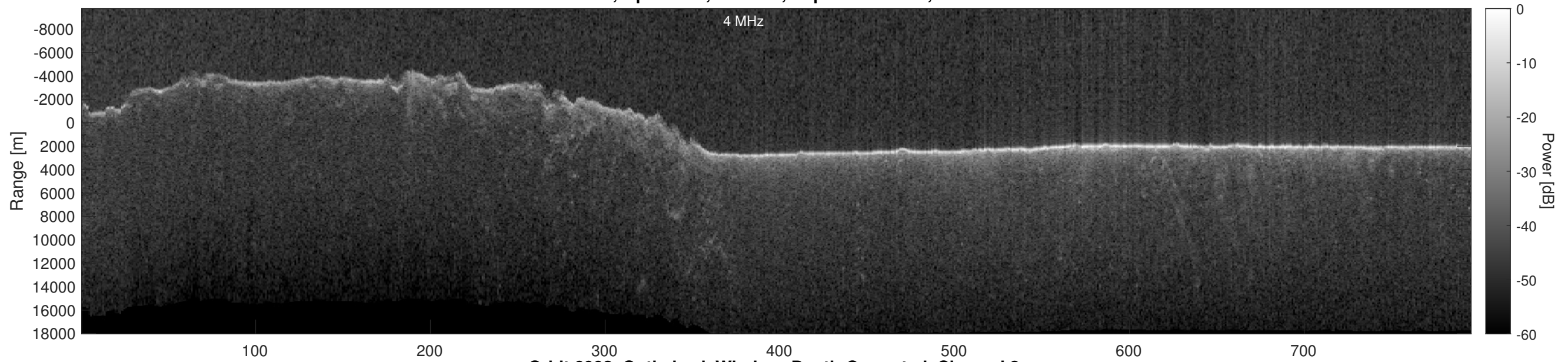
Orbit 6002, Optimized, Window, Depth-Corrected, Channel 2
