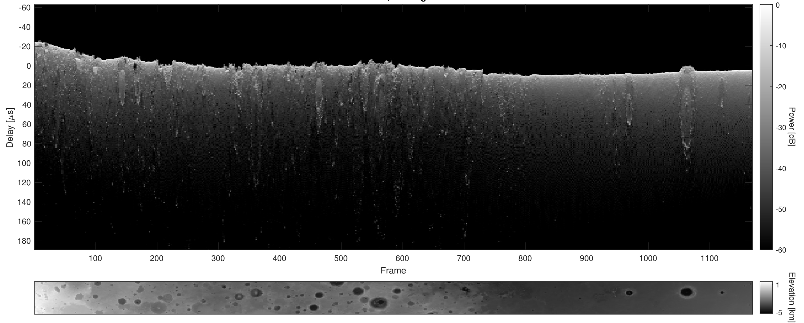
Orbit 6003, Cluttergram
