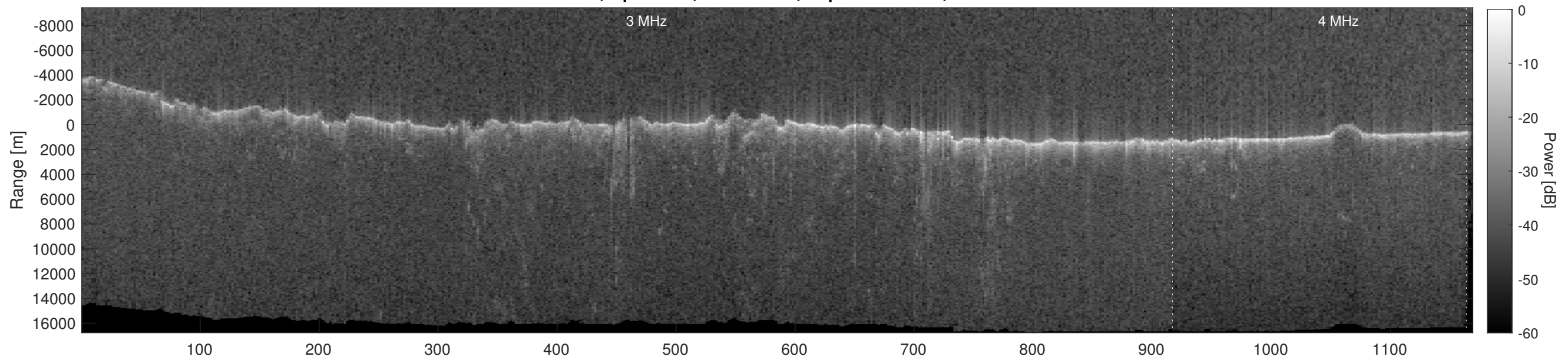
Orbit 6003, Depth-Corrected Cluttergram
