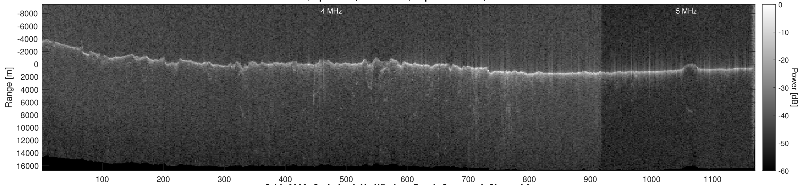
Orbit 6003, Optimized, No Window, Depth-Corrected, Channel 2
