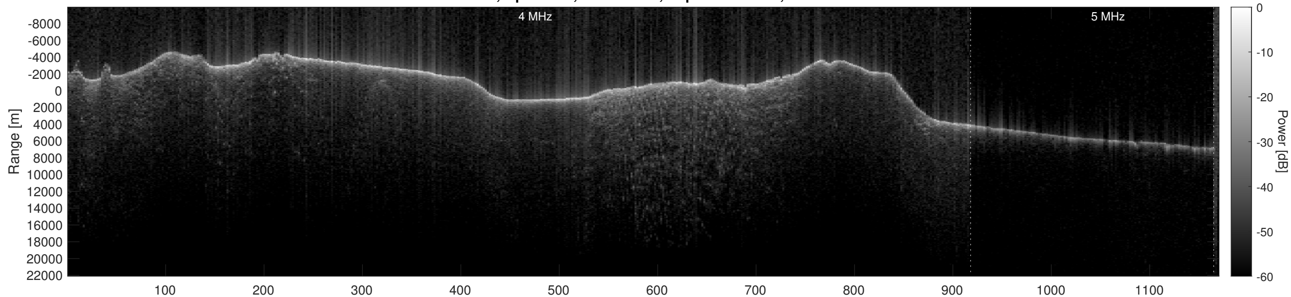
Orbit 6004, Optimized, No Window, Depth-Corrected, Channel 2
