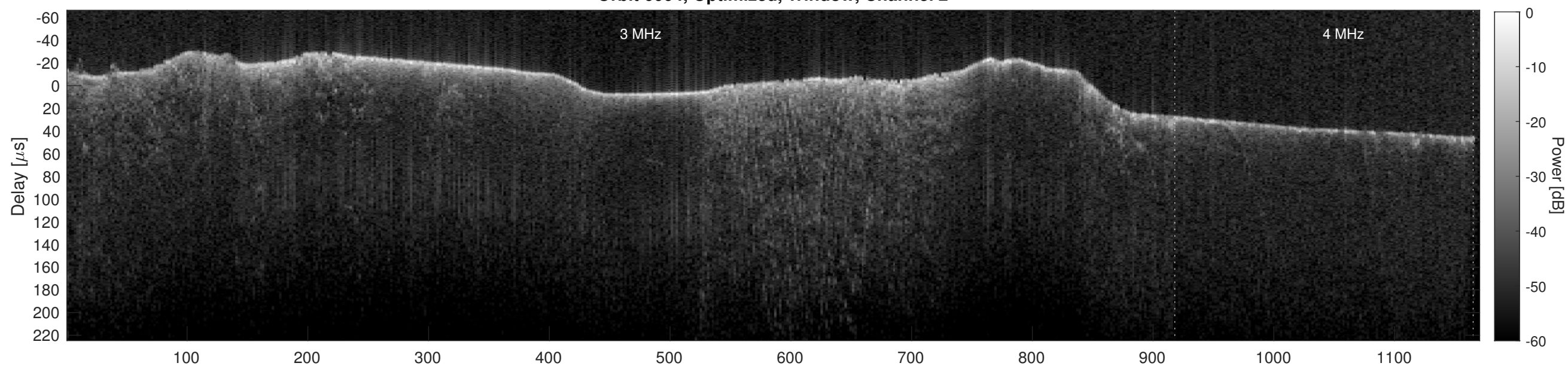
Orbit 6004, Cluttergram
