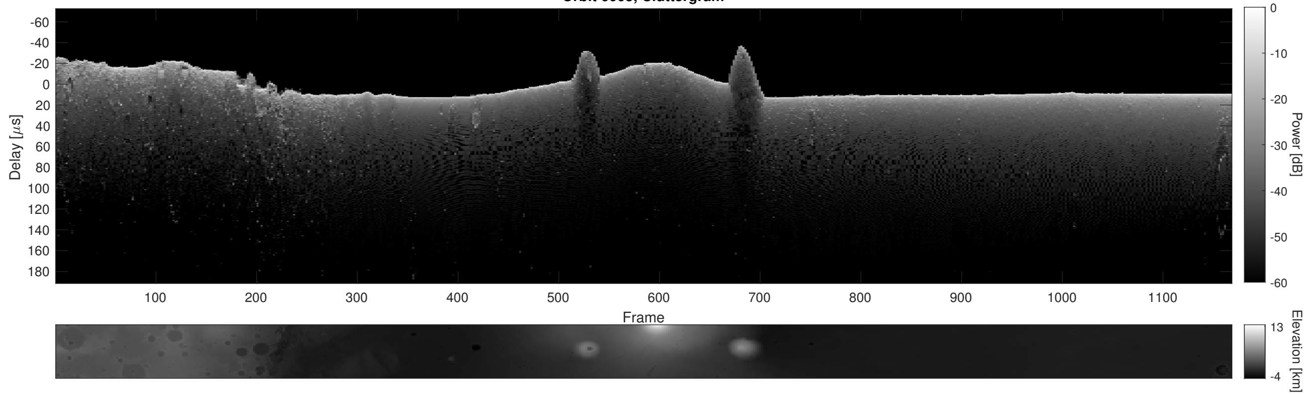
Orbit 6005, Cluttergram
