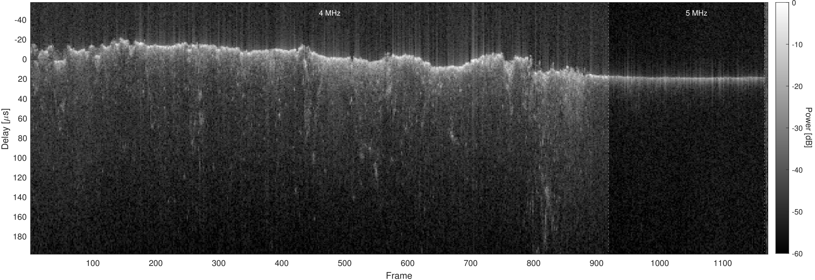
Orbit 6006, Optimized, No Window, Channel 2
