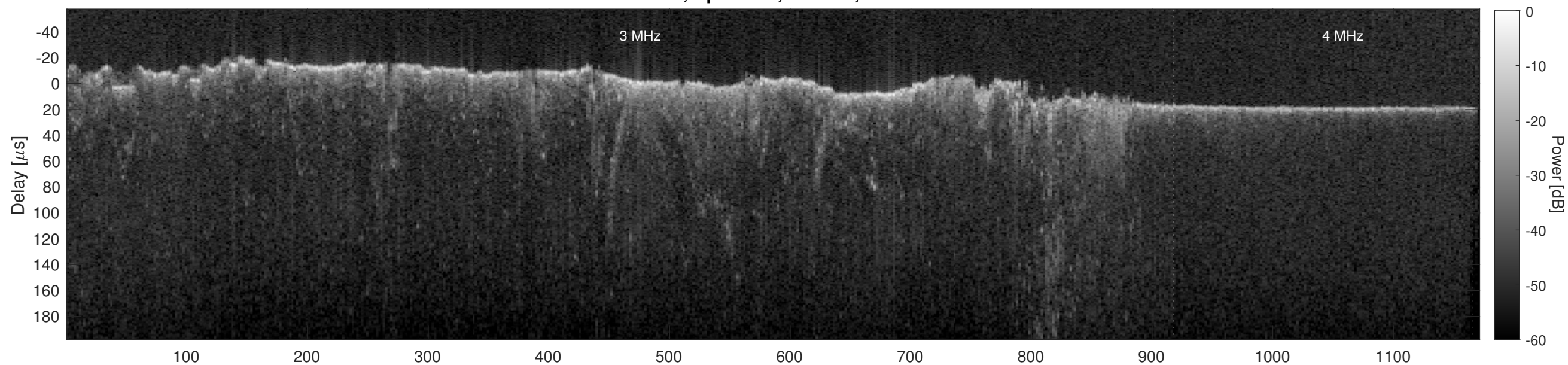
Orbit 6006, Cluttergram
