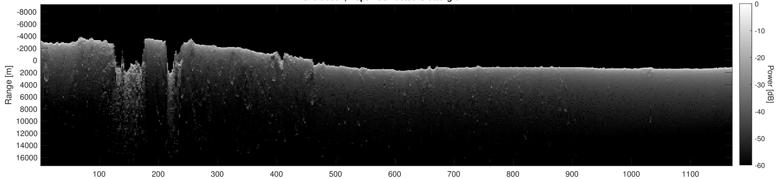
Orbit 6007, Depth-Corrected Cluttergram
