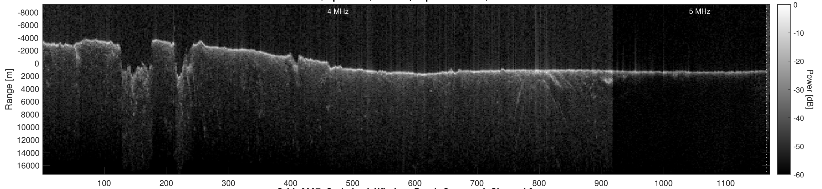
Orbit 6007, Optimized, Window, Depth-Corrected, Channel 2
