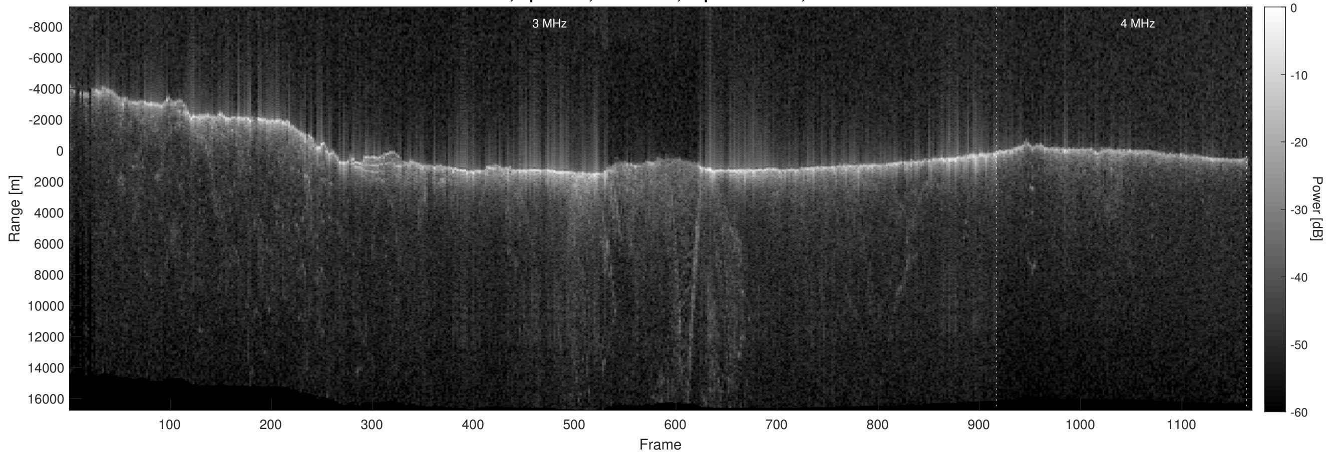
Orbit 6008, Optimized, No Window, Depth-Corrected, Channel 2
