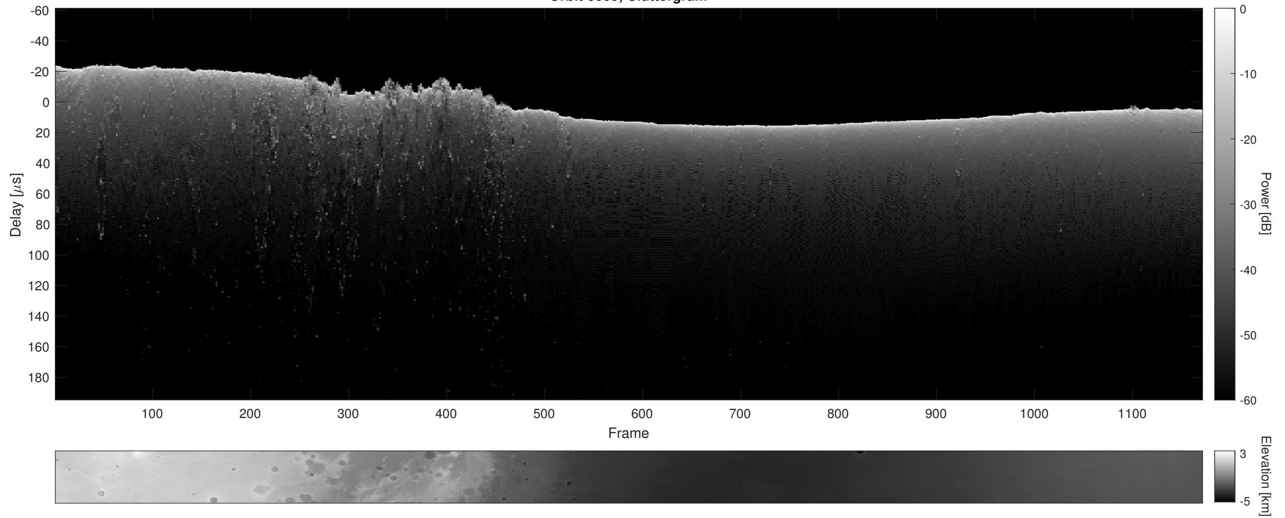
Orbit 6009, Cluttergram
