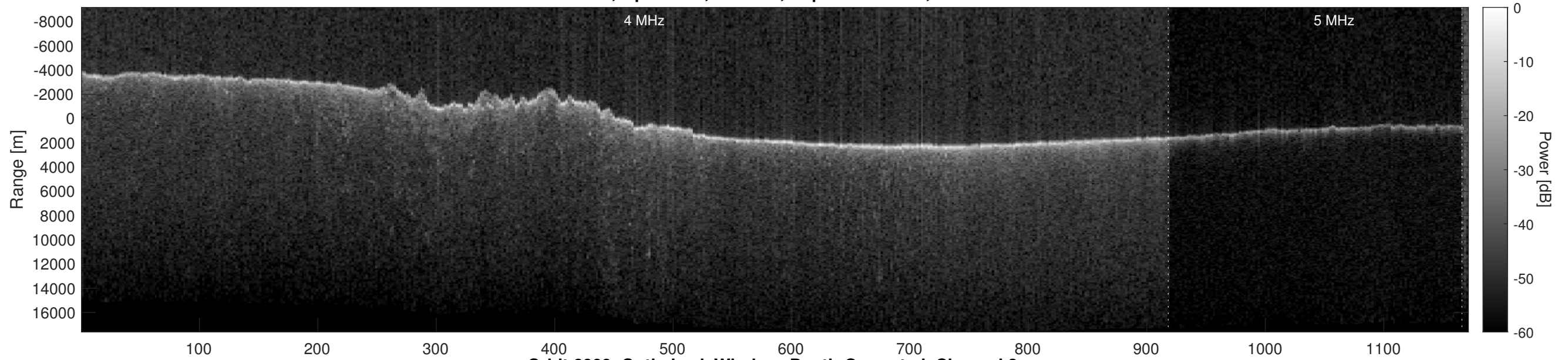
Orbit 6009, Optimized, Window, Depth-Corrected, Channel 2
