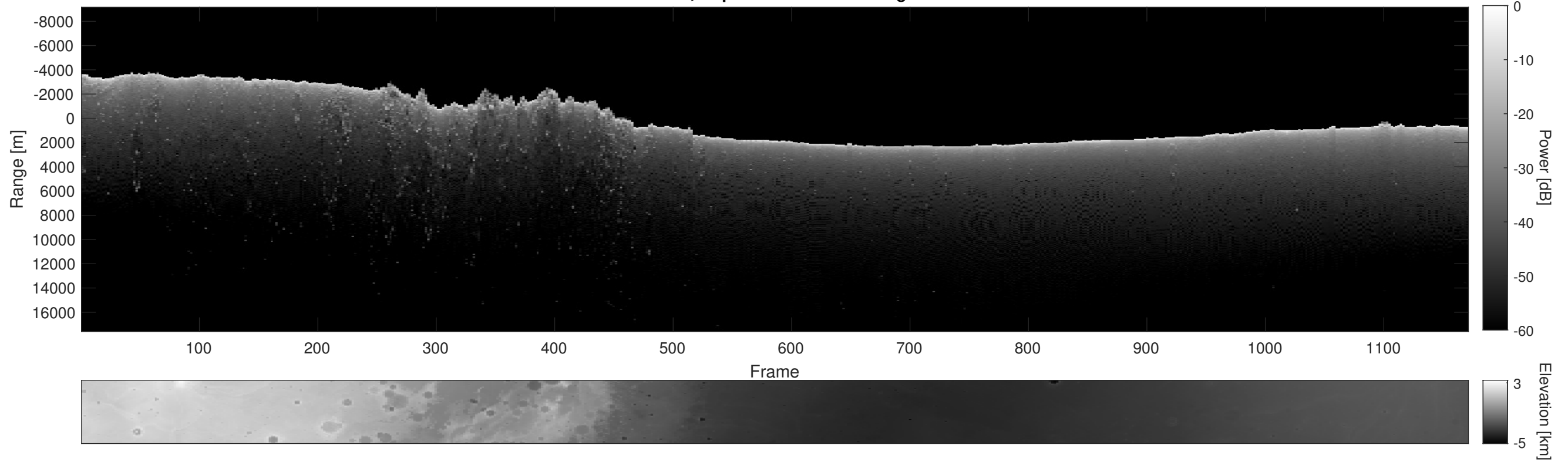
Orbit 6009, Depth-Corrected Cluttergram
