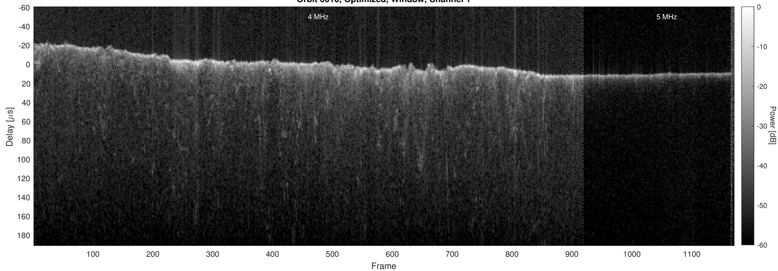
Orbit 6010, Optimized, Window, Channel 2
