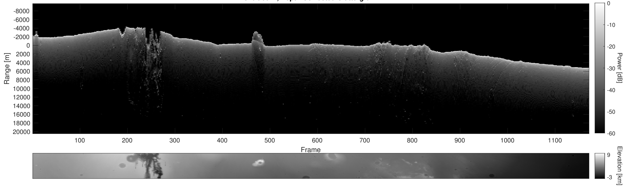
Orbit 6011, Depth-Corrected Cluttergram
