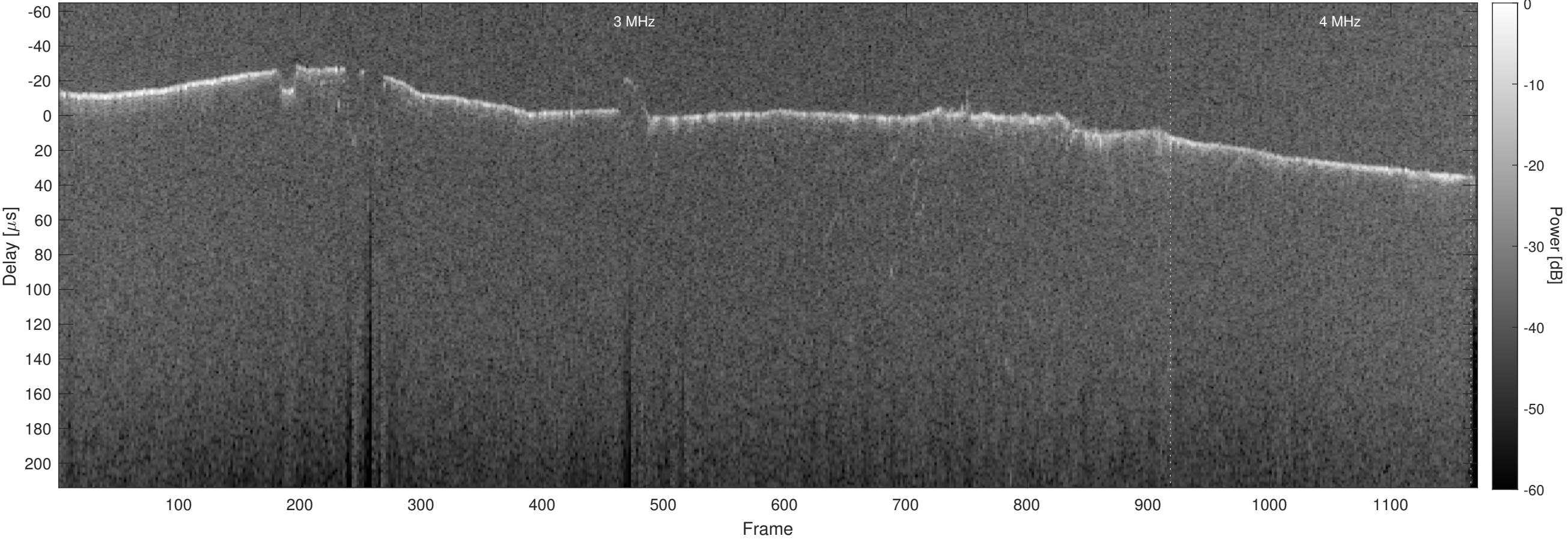
Orbit 6011, Optimized, Window, Channel 2
